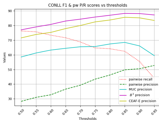
Fig. 2. Determining WD classifier threshold to maximize precision
