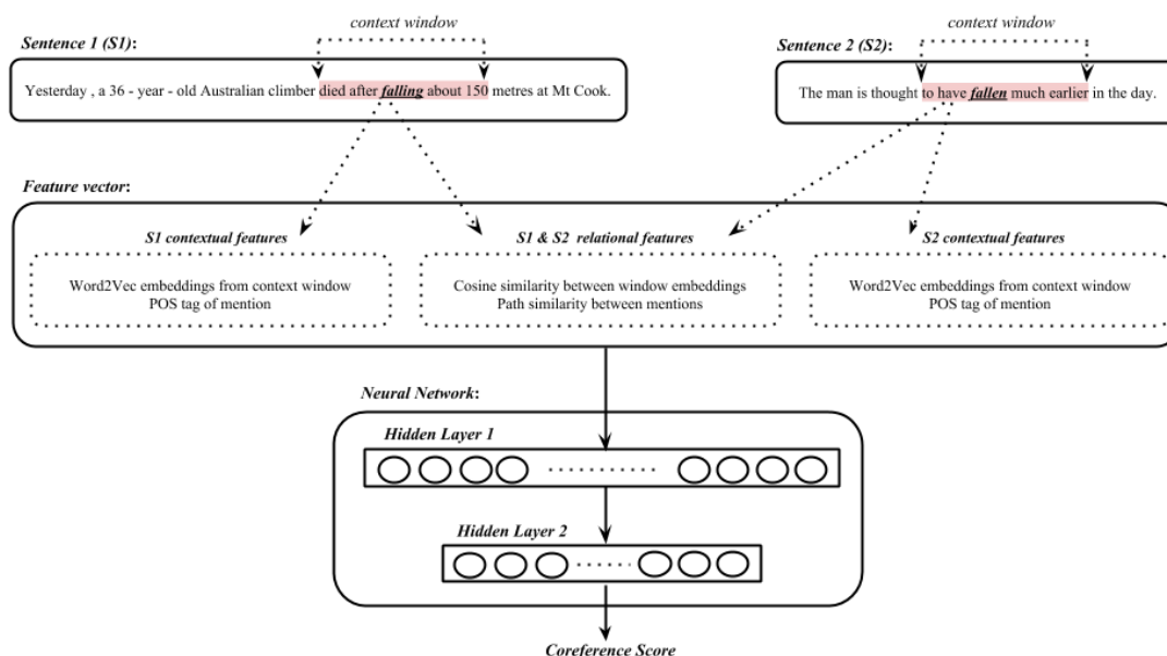
Fig. 1. Feed-forward Neural Network structure for CD resolution
