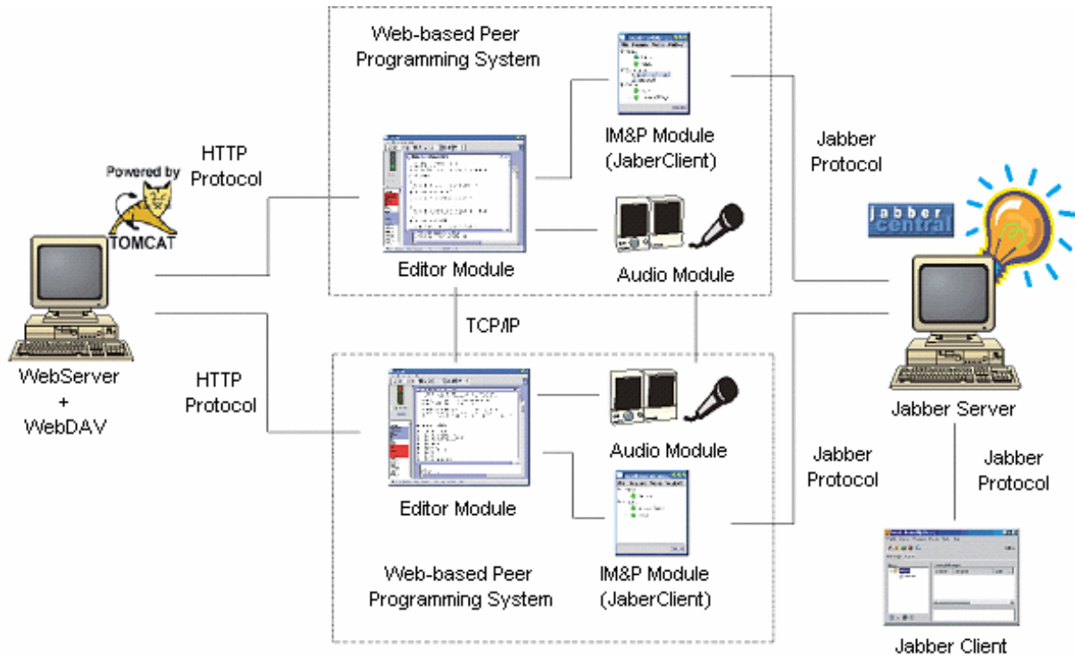
Fig. 1. Architecture of COPPER
