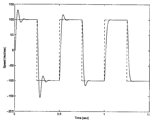
Figure 1: Speed behavior with increasing damping ( a = 75, 150, 175 ).
