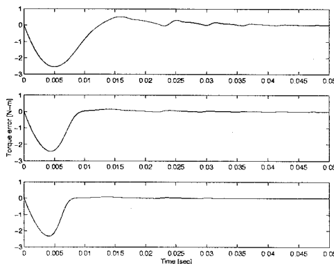
Figure 3: Torque error with increasing electric gain ( K_{vj} = 1, 5, 10 ).
