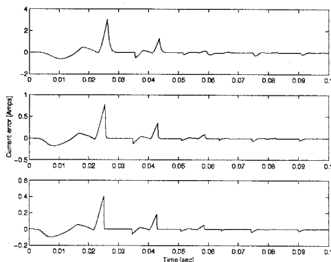
Figure 2: Current error with increasing electric gain ( K_{vj} = 1, 5, 10 ).
