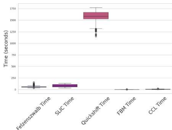
Fig. 4. Processing times running in a Ryzen 2200U for each of the algorithms under test
