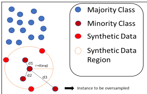
Fig. 3. The schematic diagram of Angular SMOTE algorithm for k=3
