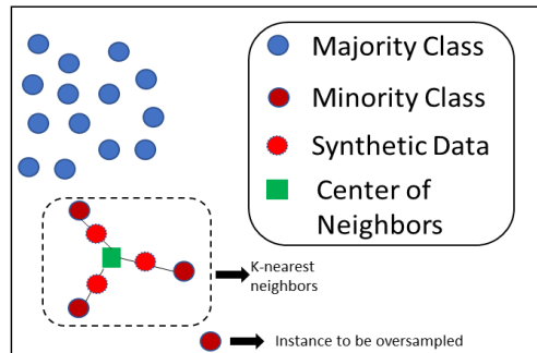
Fig. 2. The schematic diagram of Centroid-based SMOTE algorithm for k=3
