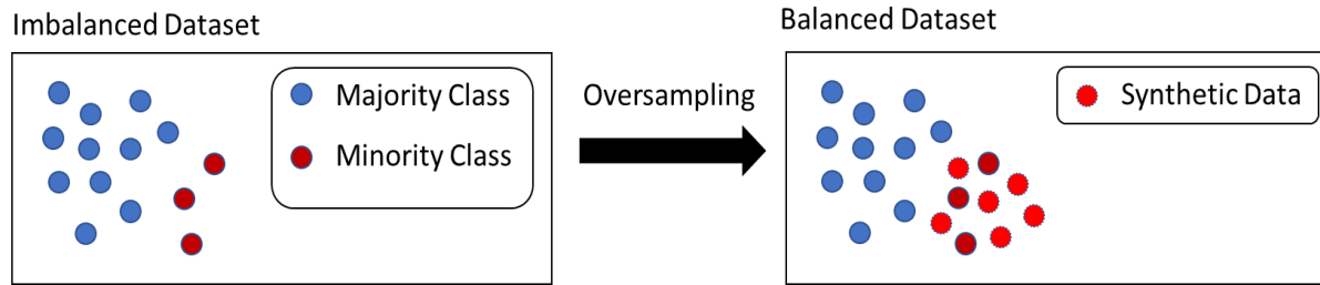
Fig. 1. Simple oversampling visualization
